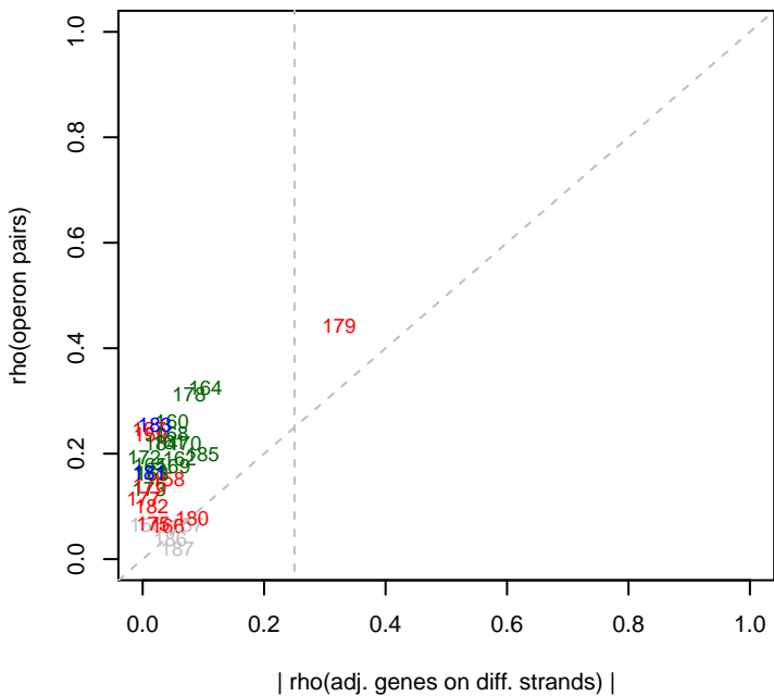
10/23/2013 Marino_ML2_set4 rho(opérons)
