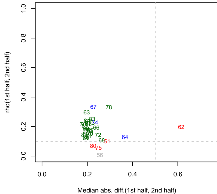
9/9/2013 Marino_ML2_set2 rho12
