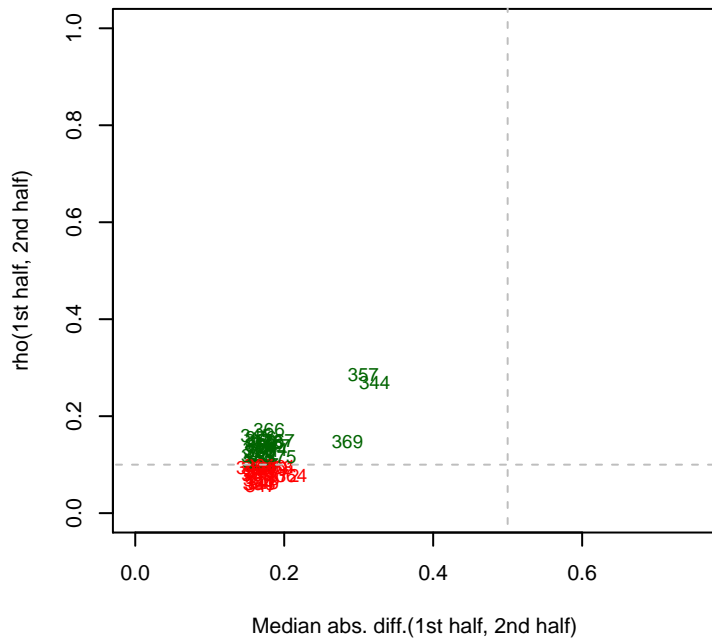
5/20/2014 Marino_ML2_set8 rho12
