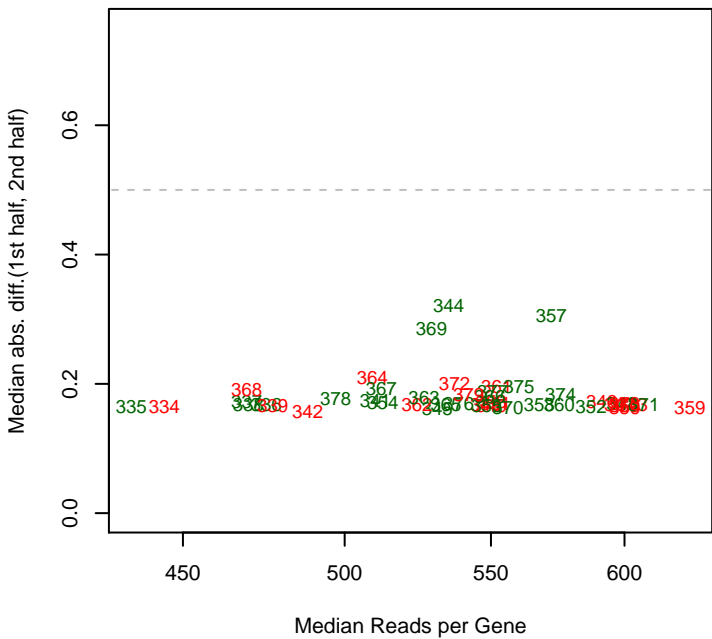
5/20/2014 Marino_ML2_set8 mad12
