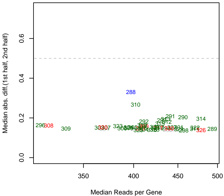
5/20/2014 Marino_ML2_set7 mad12
