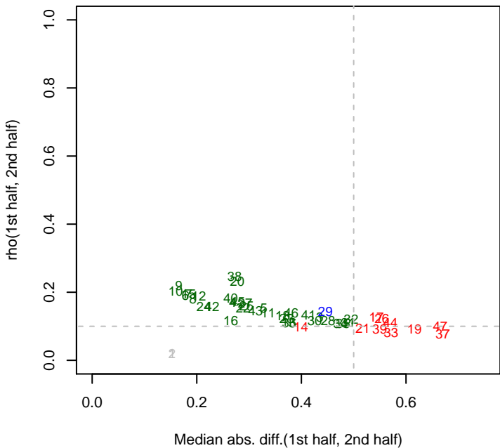
9/5/2013 Marino_ML2_set1 rho12
