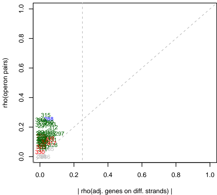
5/20/2014 Marino_ML2_set7 rho(operons)
