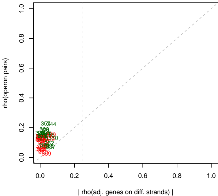
5/20/2014 Marino_ML2_set8 rho(operons)
