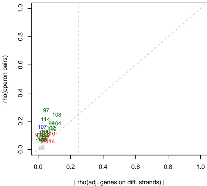
9/10/2013 Marino_ML2_set3 rho(operons)
