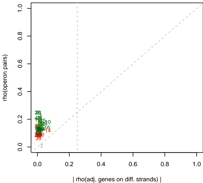
9/5/2013 Marino_ML2_set1 rho(operons)
