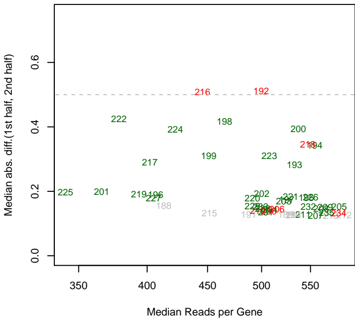
3/4/2014 Marino_ML2_set5 mad12
