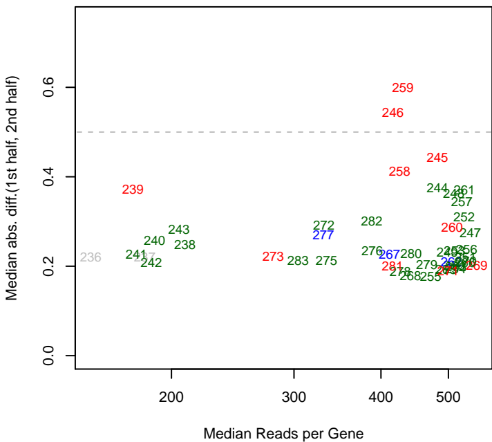
3/4/2014 Marino_ML2_set6 mad12
