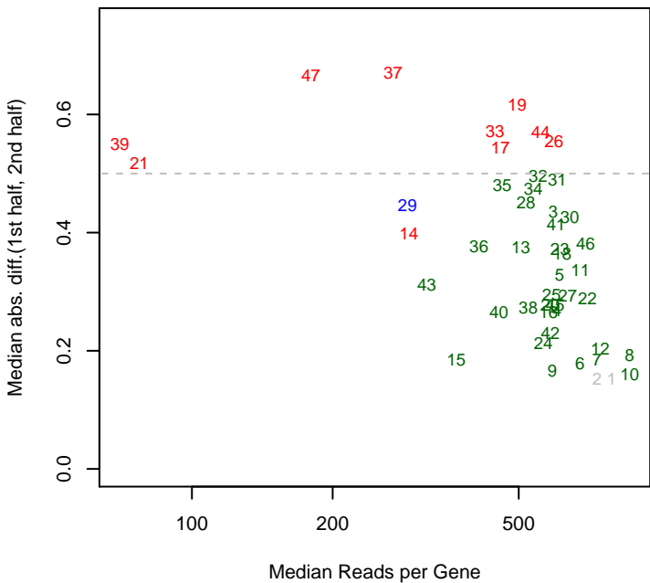
9/5/2013 Marino_ML2_set1 mad12
