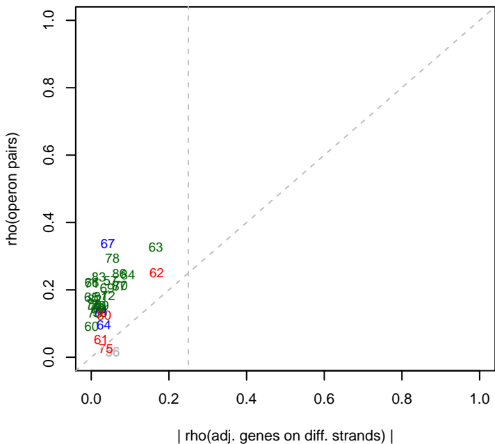
9/9/2013 Marino_ML2_set2 rho(operons)
