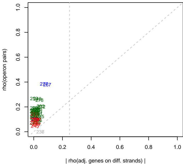
3/4/2014 Marino_ML2_set6 rho(operons)
