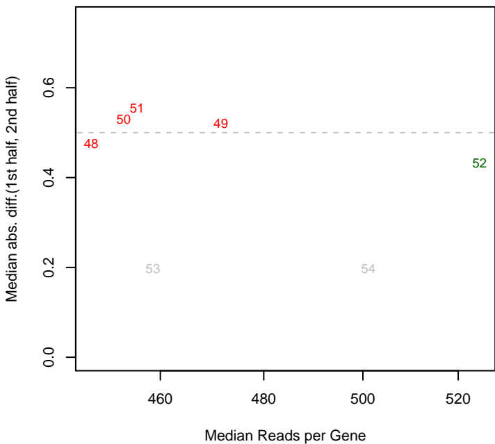
9/5/2013 Marino_ML2_set2 mad12
