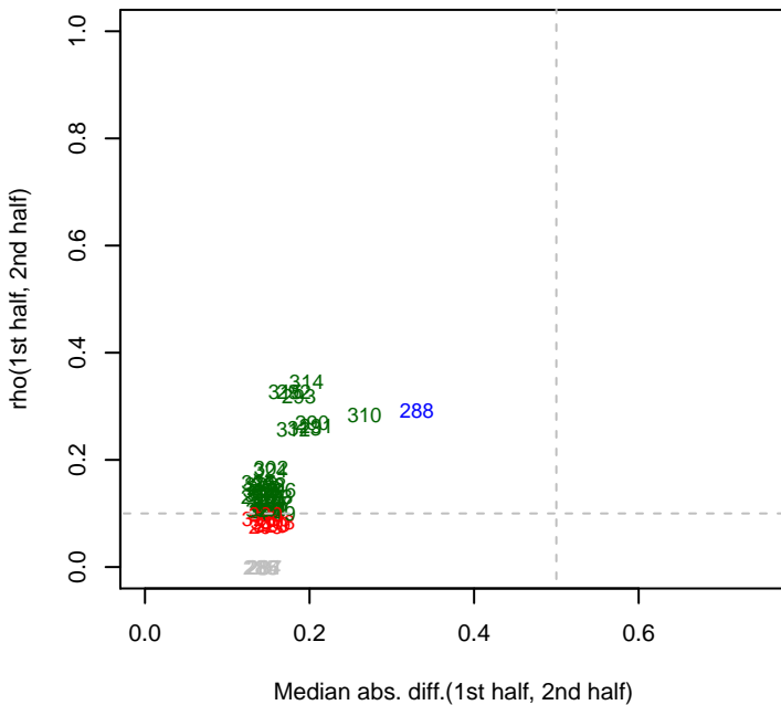
5/20/2014 Marino_ML2_set7 rho12
