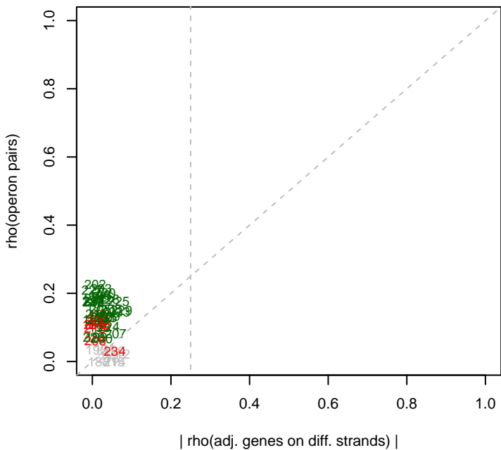
3/4/2014 Marino_ML2_set5 rho(operons)
