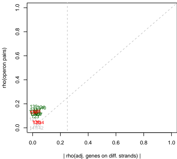
9/11/2013 Marino_ML2_set3 rho(operons)
