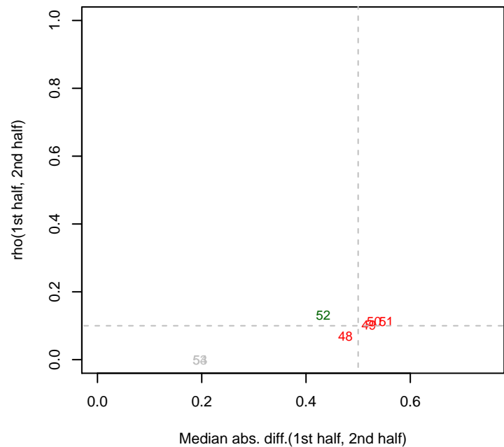
9/5/2013 Marino_ML2_set2 rho12
