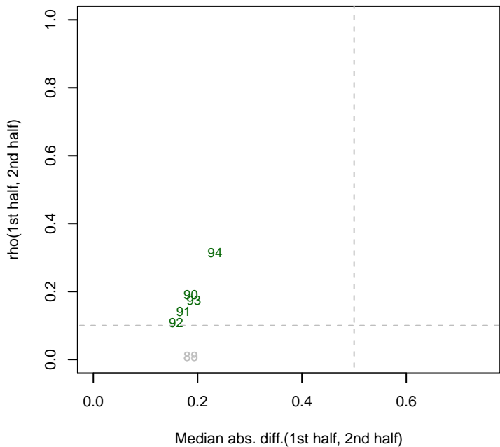
9/10/2013 Marino_ML2_set2 rho12
