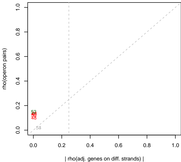
9/5/2013 Marino_ML2_set2 rho(operons)
