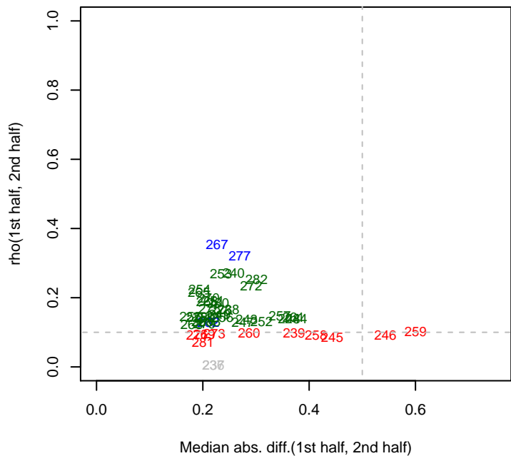
3/4/2014 Marino_ML2_set6 rho12
