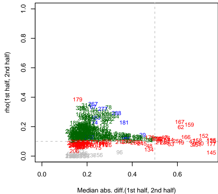
Marino rho12
