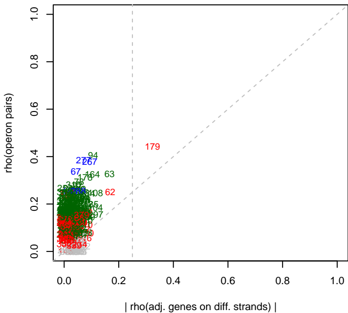
Marino rho(operons)
