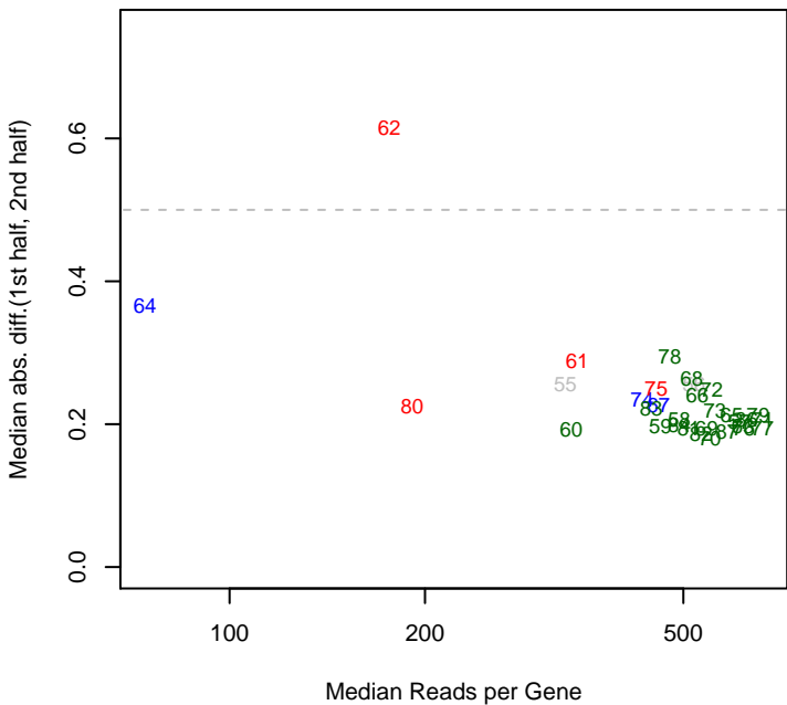
9/9/2013 Marino_ML2_set2 mad12
