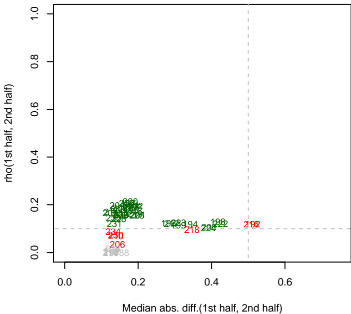
3/4/2014 Marino_ML2_set5 rho12
