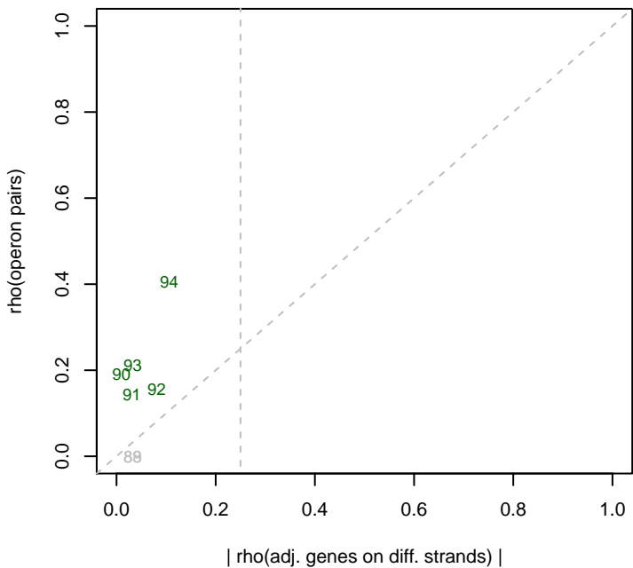
9/10/2013 Marino_ML2_set2 rho(operons)
