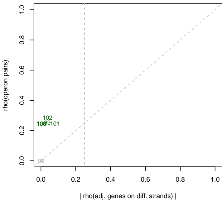
12/11/2013 PV4_ML1_set3 rho(operons)
