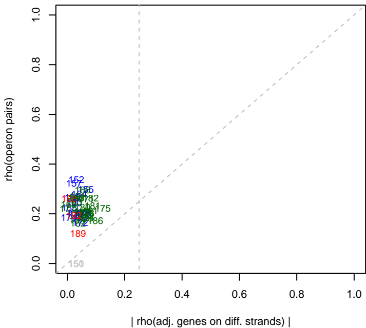
4/30/2014 PV4_ML1_set4 rho(operons)
