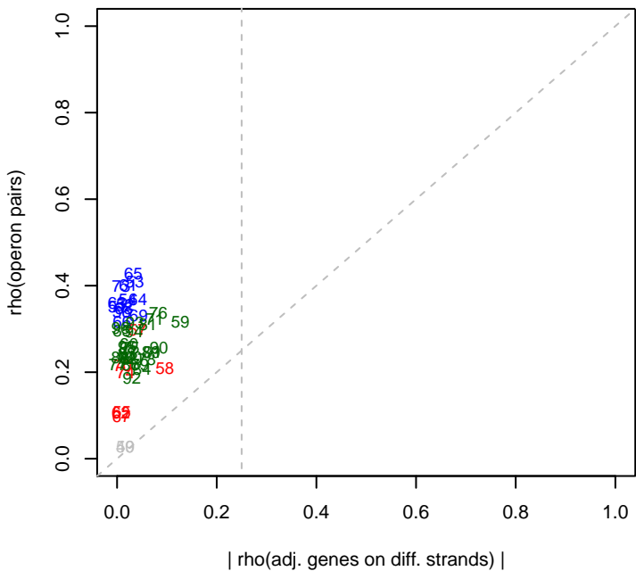
12/11/2013 PV4_ML1_set2 rho(operons)
