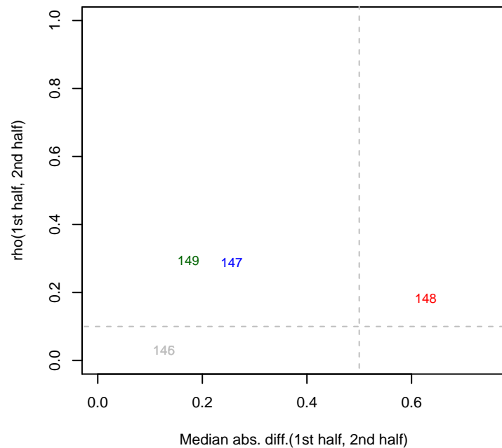
2/20/2014 PV4_ML1_set4 rho12
