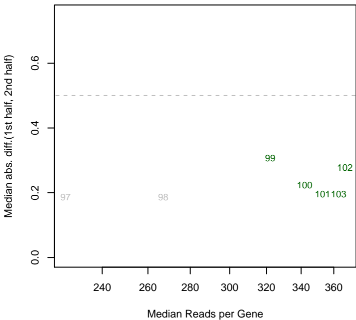
12/11/2013 PV4_ML1_set3 mad12
