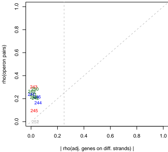
1/14/2015 PV4_ML1_set6 rho(operons)
