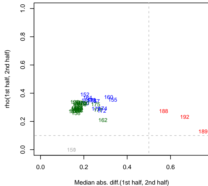
4/30/2014 PV4_ML1_set4 rho12
