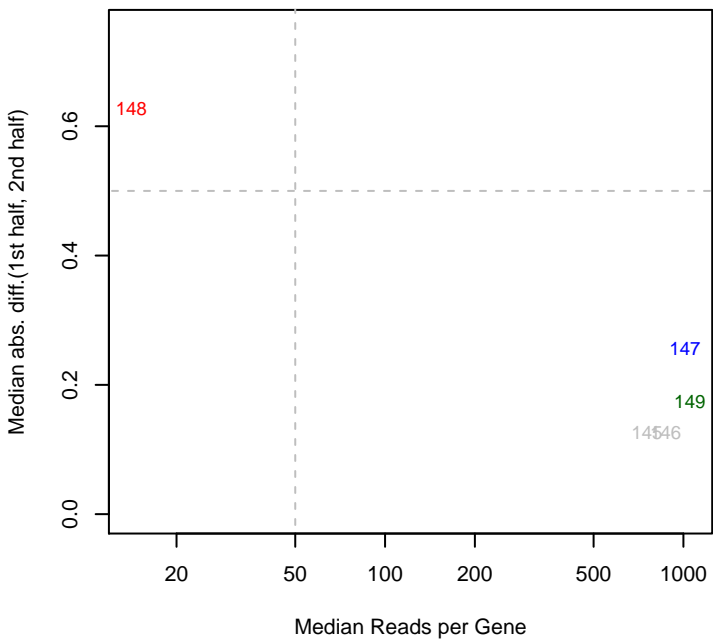
2/20/2014 PV4_ML1_set4 mad12
