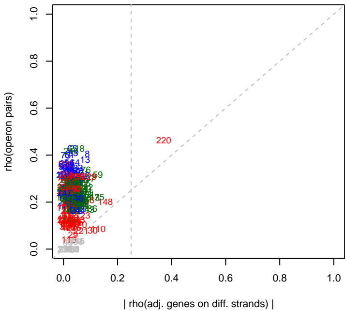
PV4 rho(operons)
