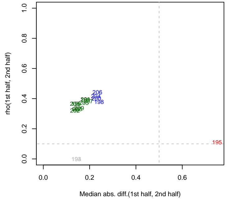
4/30/2014 PV4_ML1_set5 rho12
