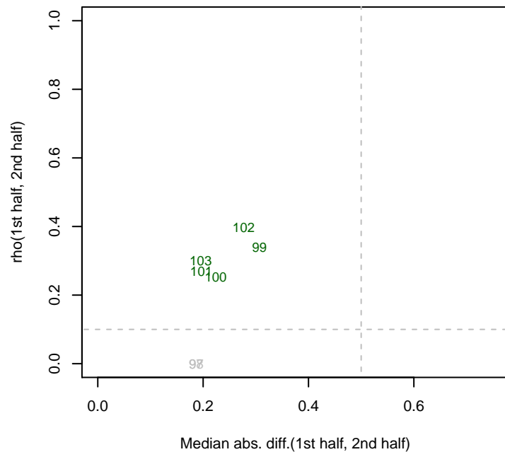
12/11/2013 PV4_ML1_set3 rho12
