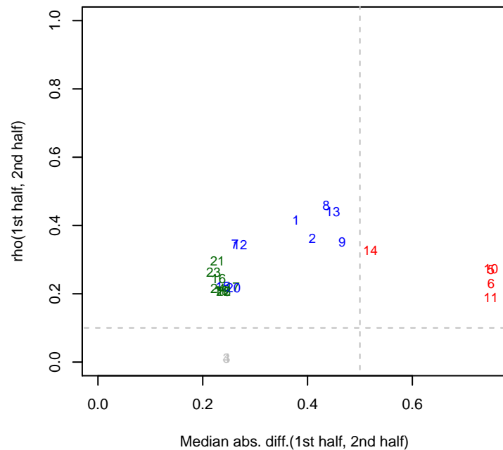
12/11/2013 PV4_ML1_set1 rho12
