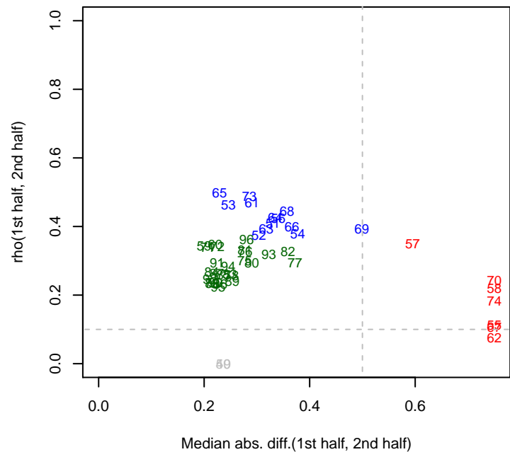
12/11/2013 PV4_ML1_set2 rho12
