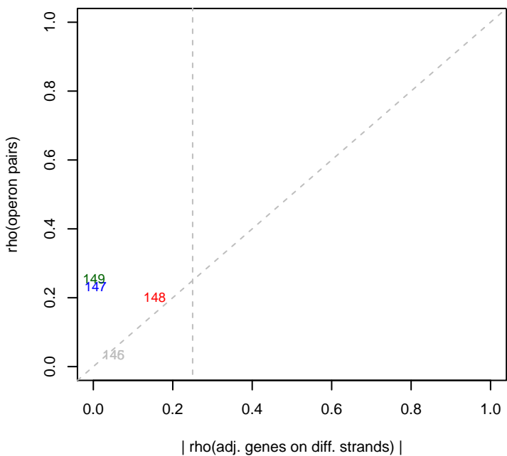
2/20/2014 PV4_ML1_set4 rho(operons)
