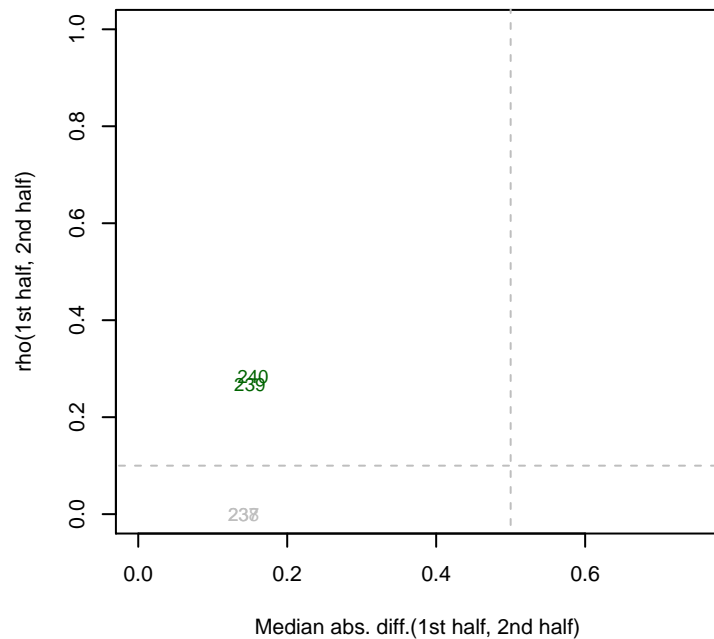
12/11/2013 PV4_ML1_set5 rho12
