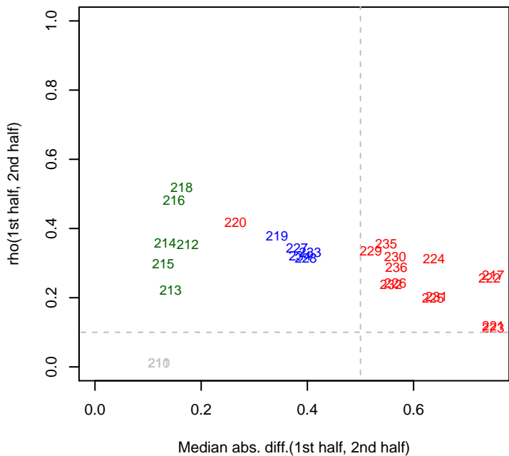
8/28/2013 PV4_ML1_set5 rho12
