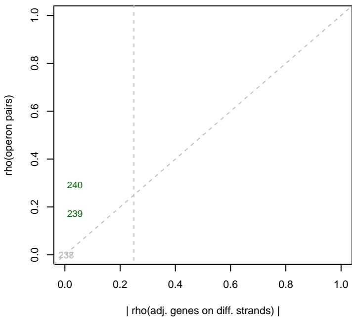
12/11/2013 PV4_ML1_set5 rho(operons)
