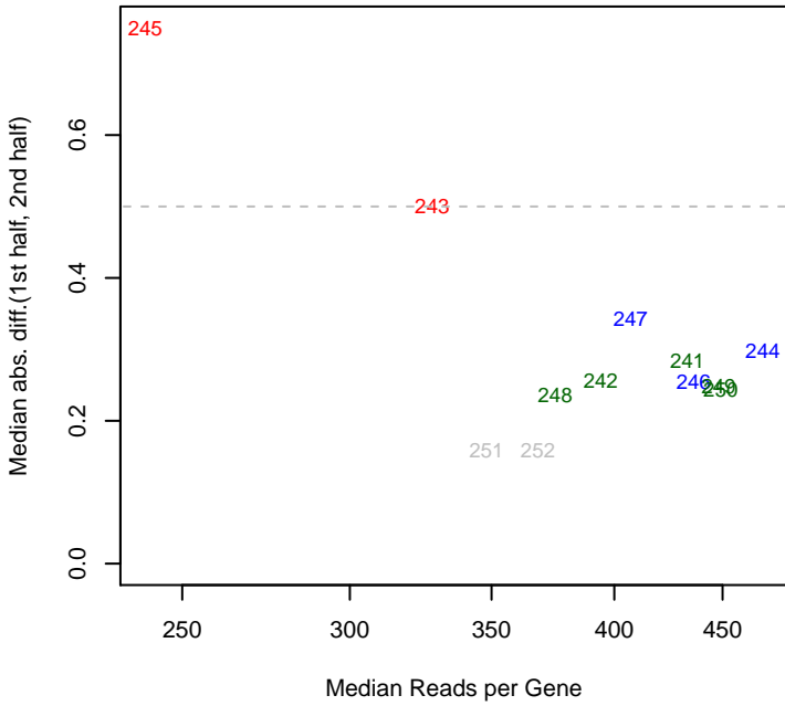
1/14/2015 PV4_ML1_set6 mad12
