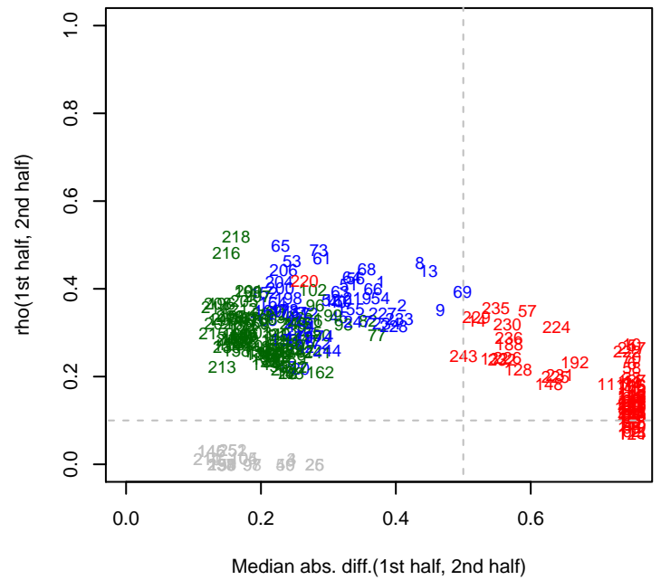
PV4 rho12
