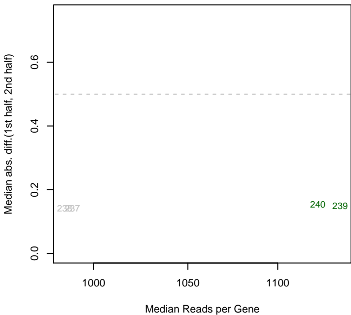
12/11/2013 PV4_ML1_set5 mad12
