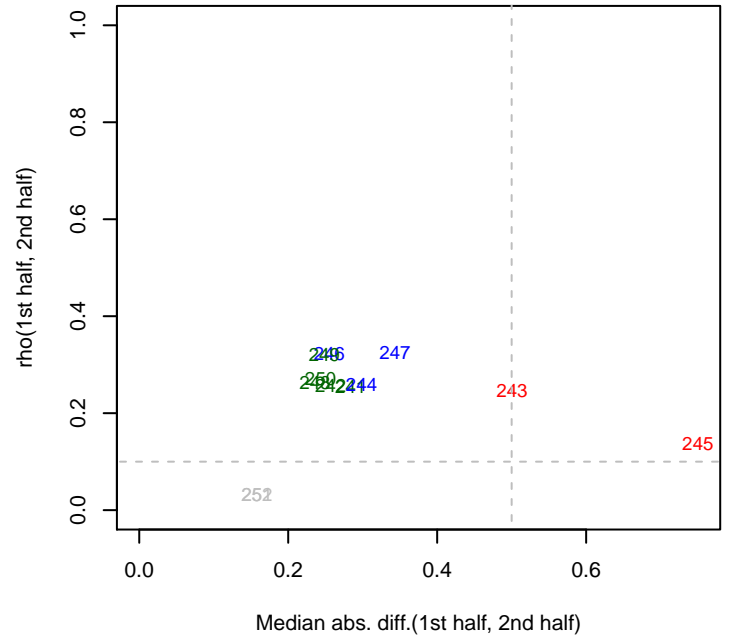
1/14/2015 PV4_ML1_set6 rho12
