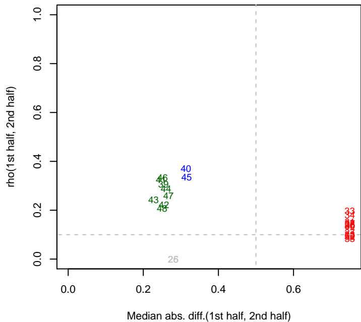
2/20/2014 PV4_ML1_set1 rho12
