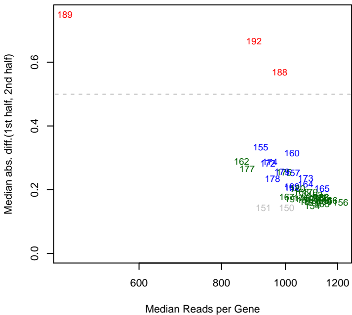
4/30/2014 PV4_ML1_set4 mad12
