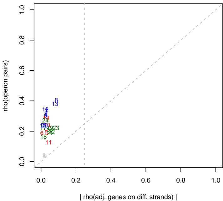
12/11/2013 PV4_ML1_set1 rho(operons)
