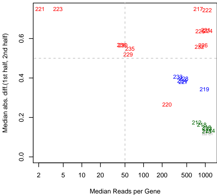
8/28/2013 PV4_ML1_set5 mad12
