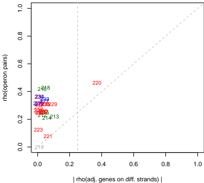
8/28/2013 PV4_ML1_set5 rho(operons)
