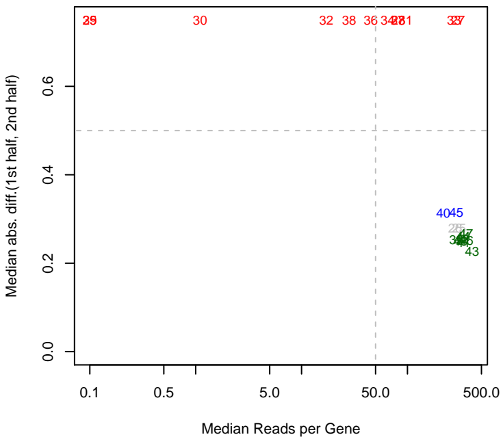
2/20/2014 PV4_ML1_set1 mad12
