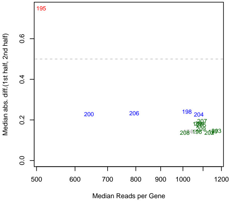
4/30/2014 PV4_ML1_set5 mad12
