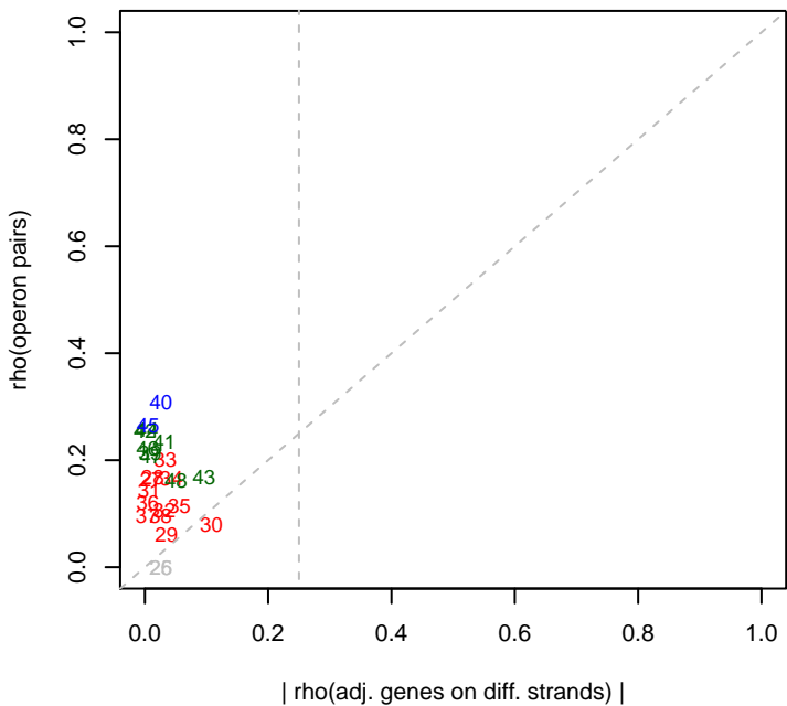
2/20/2014 PV4_ML1_set1 rho(operons)
