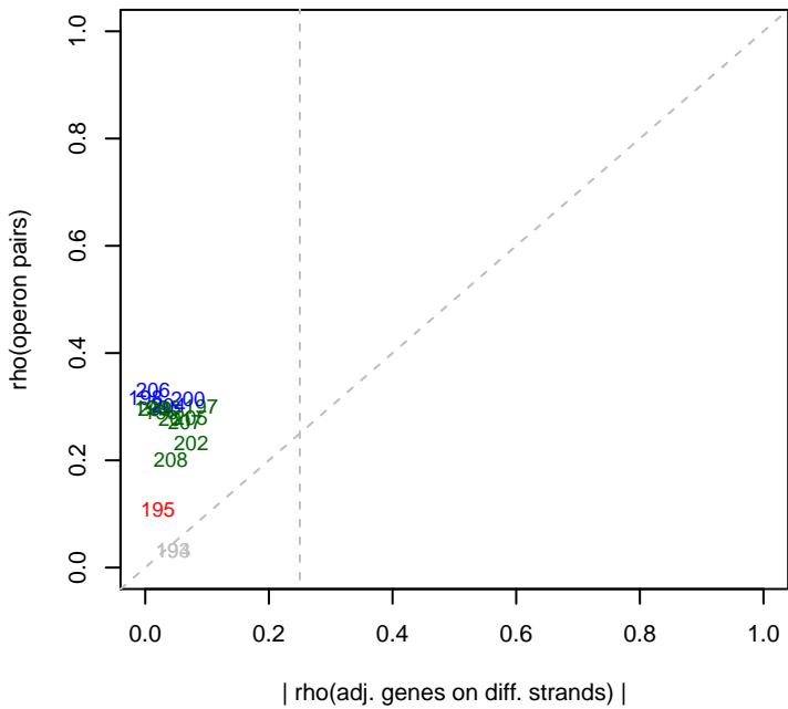
4/30/2014 PV4_ML1_set5 rho(opérons)
